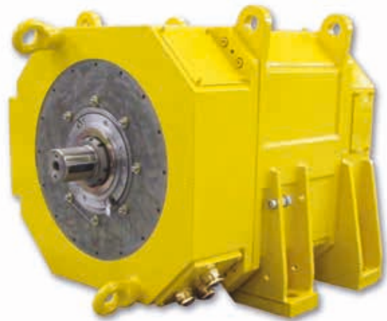
Figure 2. WL16BC080 'short' high power density drilling motor delivers 800 hp in a standard 600 hp frame and comes in vertical and horizontal configurations.
