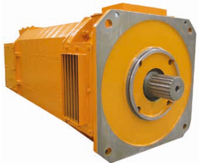
Figure 3. WL13BB080 'long' high power density drilling motor delivers up to 33% more torque and horsepower within the same standard 600 hp frame size.
